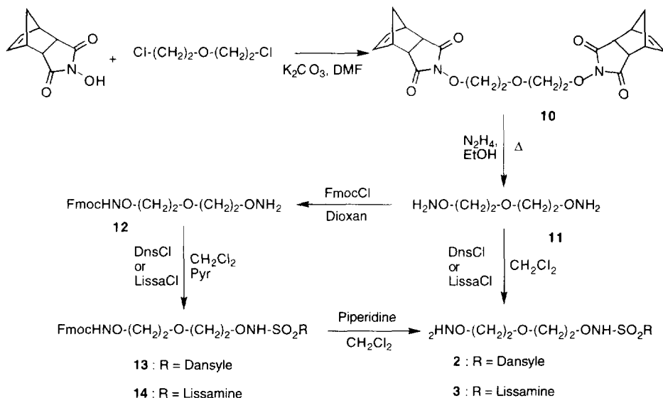
Scheme 2: Synthesis of probes 2 and 3
