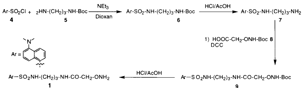
Scheme 1 : Synthesis of compound 1
